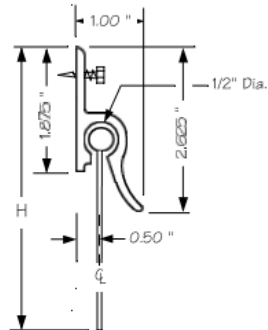
HEAVY DUTY FLAT WALL BONDED BEAD
