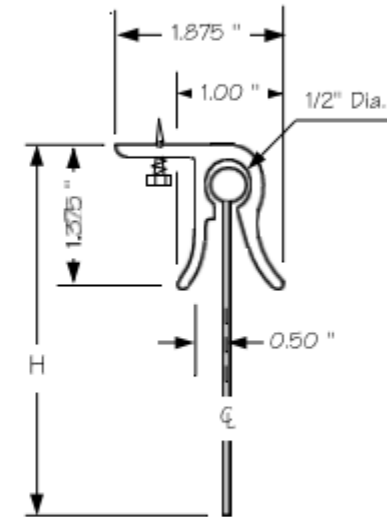
HEAVY DUTY IN JAMB BONDED BEAD
